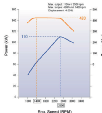
N04C-US Powerband
